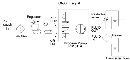
Fig 3. Circuit Example
