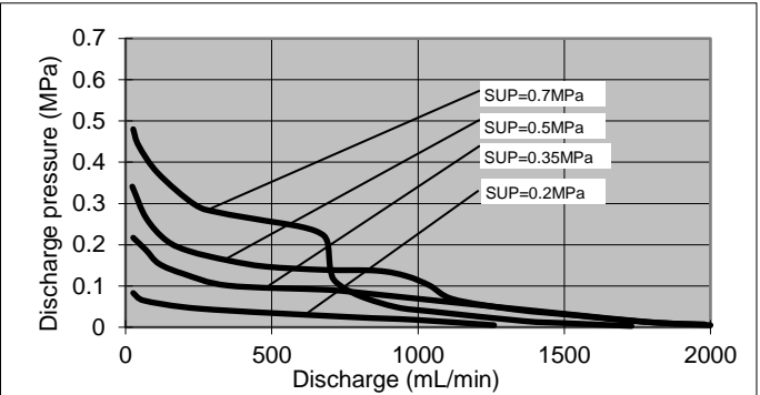
Fig 1c. Flow rate characteristic graph for Cycle (7Hz)
