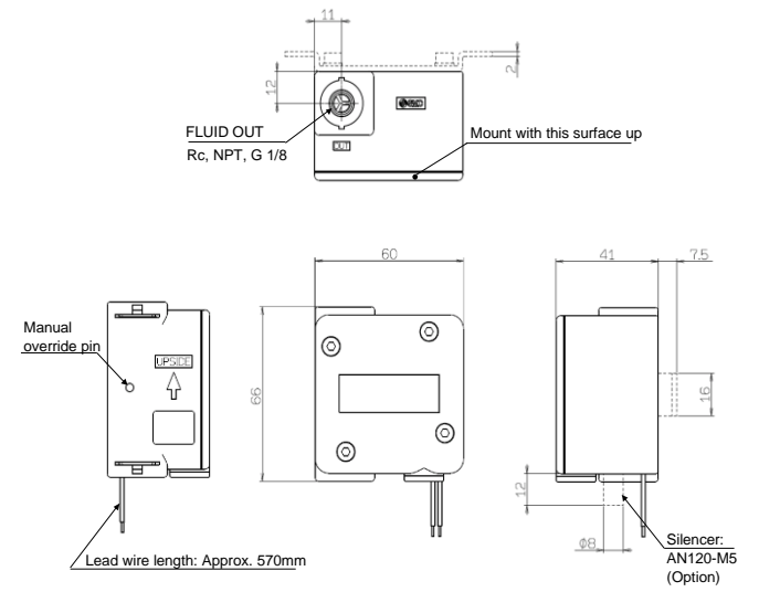
Fig 4. Outline dimensions
