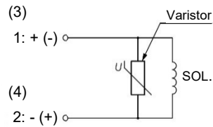
Figure 10. Grommet / DIN terminal / Conduit with surge voltage suppressor / M12 connector (3,4)
