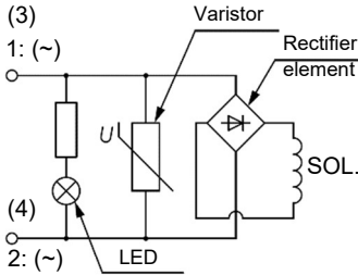
Figure 12. DIN terminal with LED and surge voltage suppressor
