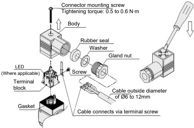
Figure 6. DIN connector construction
